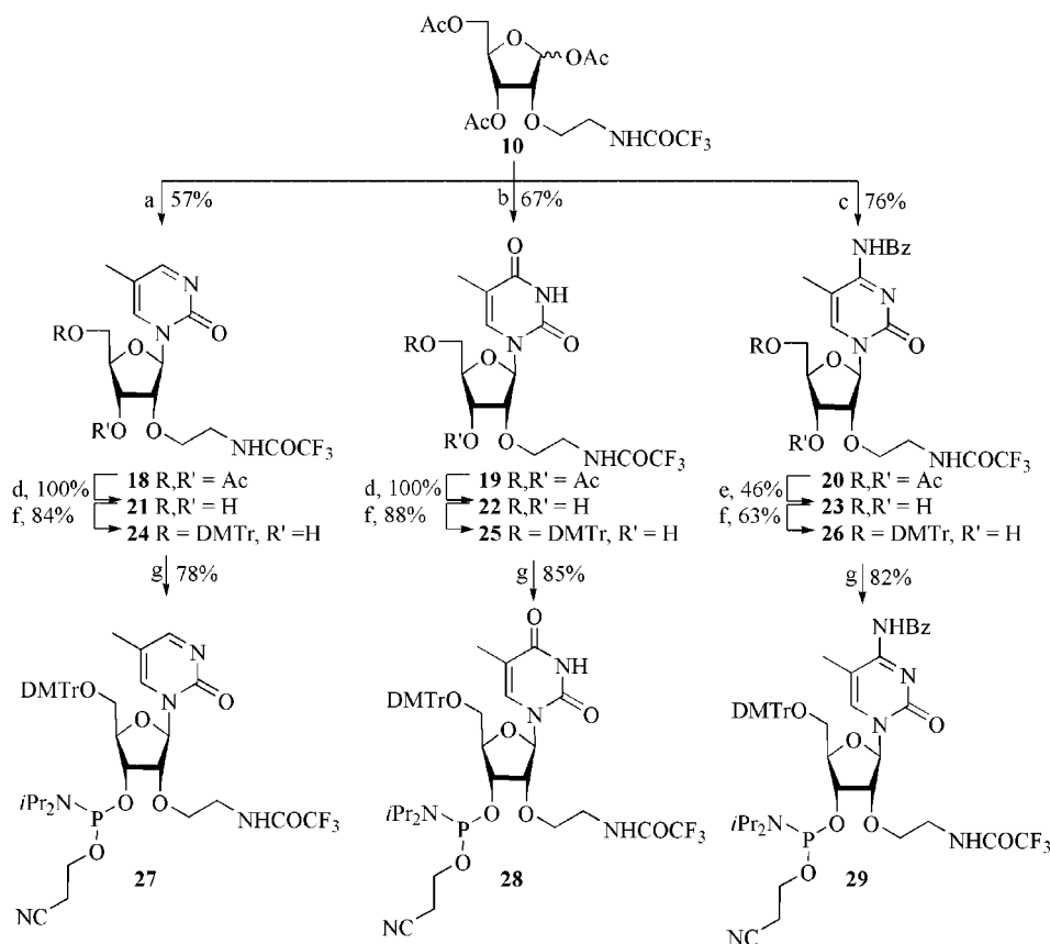
Scheme 3. Synthesis of nucleosides and phosphoramidites 27–29 . a) 13 , BSA, SnCl 4 , CH 3 CN, 2 h, 0 °C. b) 14 , BSA, SnCl 4 , CH 3 CN, 4 h, 0 °C → room temp. c) 17 , HMDS, TMS-Cl, TMS-Tf, CH 3 CN, 2 h, room temp. d) Na 2 CO 3 , MeOH, 15 min to 2 h, room temp. e) 50% ethanolic solution of NaOH (2 N NaOH/EtOH, 1:1), pyridine/EtOH, 1:2, 5–20 min, room temp. f) DMT-Cl, pyridine, 3 to 6 h, room temp. g) i Pr 2 NEt, CEP-Cl, THF, 2 to 3 h, room temp.
