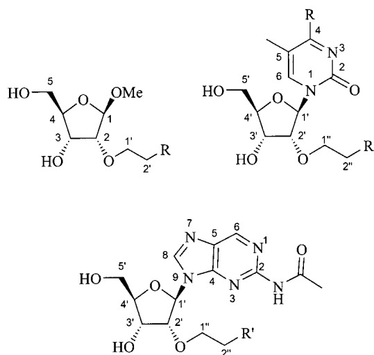
Numbering scheme for compounds 2–10 and 18–37
