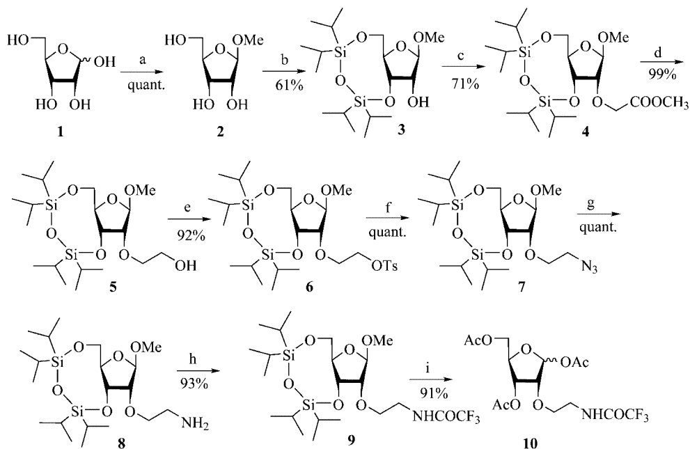
Scheme 1. Synthesis of the sugar building block 9 . a) Dowex-50 H + , MeOH, overnight, 4 °C. b) TIPS-Cl, pyridine, 1 h, room temp. c) BrCH 2 CO 2 Me, NaH, DMF, 7 h, −10 °C → room temp. d) LiBH 4 , THF/MeOH, 40 min, 0 °C. e) TsCl, NEt 3 , DMAP, CH 2 Cl 2 , overnight, room temp. f) LiN 3 , DMF, 1 h, 100 °C. g) i. Ph 3 P, pyridine, 3 h, room temp. ii. NH 3 33%, 4 h, room temp. h) Et 3 N, CF 3 CO 2 Et, 4 h, room temp. i) Ac 2 O/AcOH/H 2 SO 4 , overnight, room temp.
