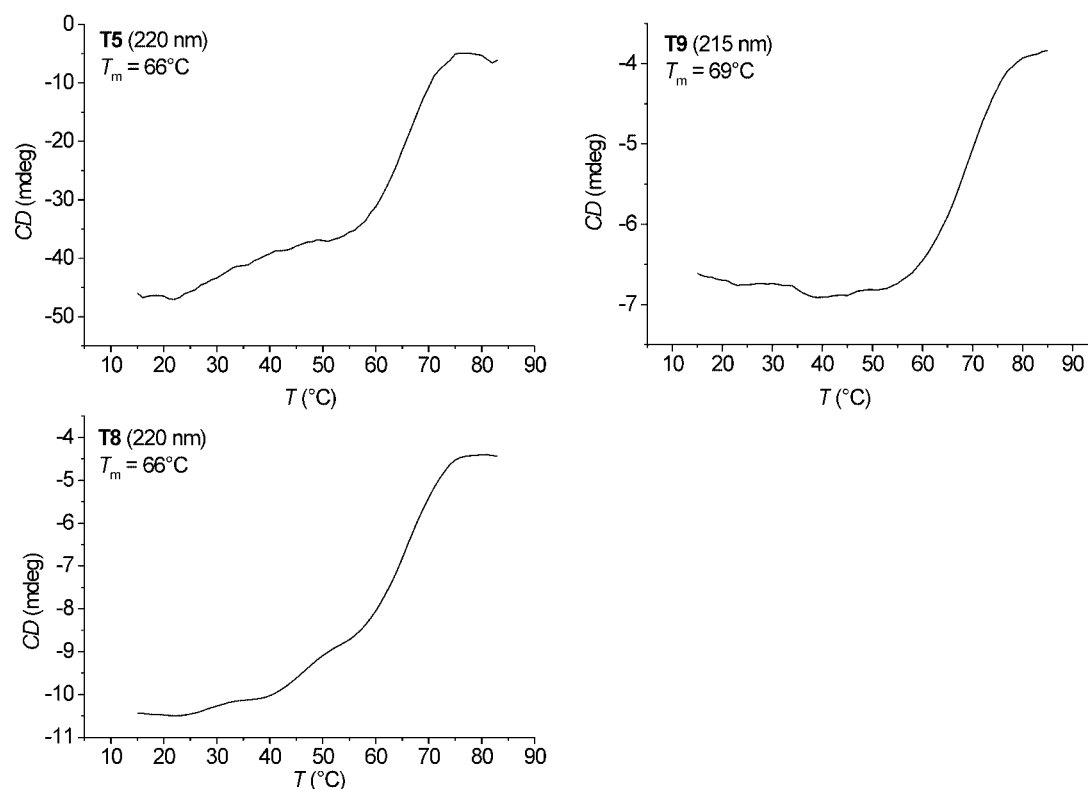
Figure 3. CD melting curves of triplex T5 (top, left) T8 (bottom left) and T9 (top, right) at the indicated wavelength. Buffer: c (single strand) = 1.6 \mu\text{M} ( T5 ), 3.8 \mu\text{M} ( T8 ) and 1.6 \mu\text{M} ( T9 ) in 10 mM sodium cacodylate, 100 mM NaCl, 0.25 mM spermine, pH 7.0.
