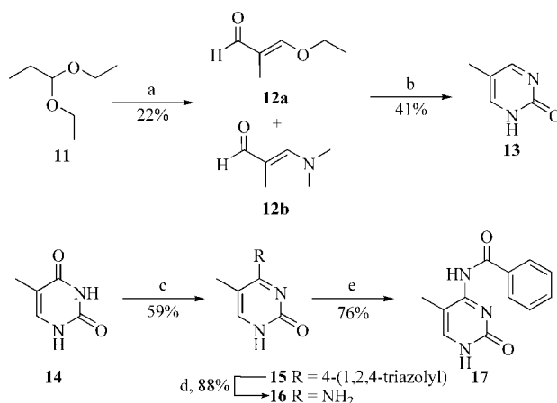
Scheme 2. Synthesis of bases. a) i. POCl 3 , DMF, 2 h, 70 °C. ii. H 2 O, K 2 CO 3 , overnight. b) i. Na, Urea, EtOH, 2 d, reflux. ii. HCl 25%, 1 d, reflux. c) POCl 3 , Et 3 N, 1 H -1,2,4-triazole, CH 3 CN, 5–7 h, room temp. → reflux. d) NH 3 33%, 3 h, reflux. e) Bz 2 O, DMAP, CH 3 CN, 7 h, reflux.
