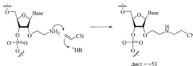
Scheme 5. Proposed mechanism for the reaction of acrylonitrile with the amino side chain.
