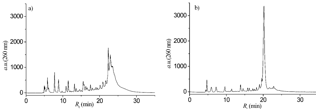
Figure 2. RP-HPLC traces of TFO T2 : comparison between two different deprotection protocols. a) standard: \text{NH}_3 33%, room temp., 2 h. b) modified: DBU 1 M in \text{CH}_3\text{CN} , room temp., 2 h followed by \text{NH}_3 33%, room temp., 2 h.
