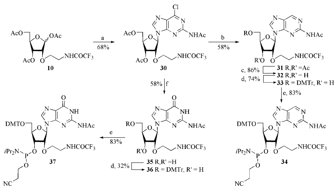
Scheme 4. Synthesis of phosphoramidites 34 and 37 . a) i) 2-aminoacetyl-6-chloropurine, BSA, ClCH 2 CH 2 Cl, 80 °C, 20 min. ii) 1 , TMSOTf, toluene, 80 °C, 3 h. b) Et 3 N, Pd/C, H 2 , EtOAc, room temp., 5 h. c) Na 2 CO 3 , MeOH, 1 h, room temp. d) DMT-Cl, mol. sieves, pyridine, 4 h, room temp. e) i Pr 2 NEt, CEP-Cl, mol. sieves, THF, 1.5 to 3 h, room temp., 83%. f) NC(CH 2 ) 2 OH, Cs 2 CO 3 , THF, 0 °C, 2 h.
