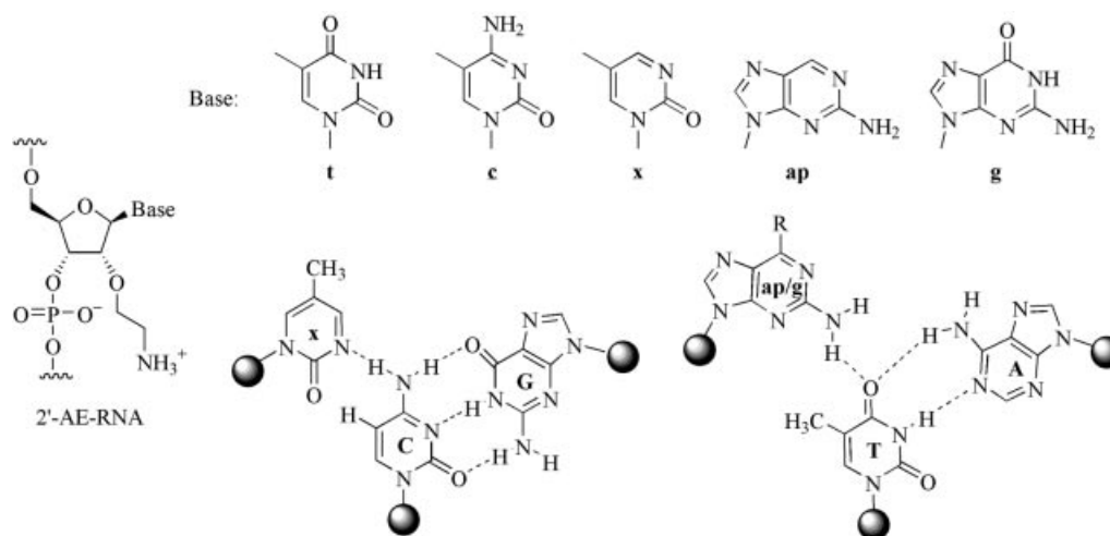
Figure 1. Chemical structures of the 2'-AE nucleotides prepared and used in this study together with the putative x-CG, and g/ap-TA base triple.
